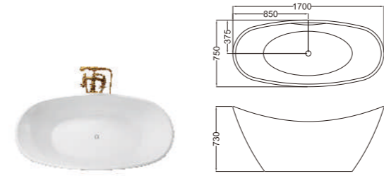
C-3026 Size:750x1700x730/mm
