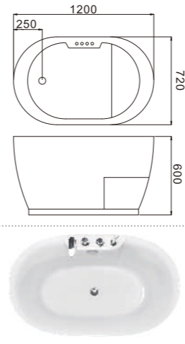
C-3250 Size:720x1200x600/mm
