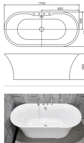
C-3224 Size:780x1700x580/mm
