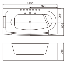
C-468 Size:900x1850x580/mm
