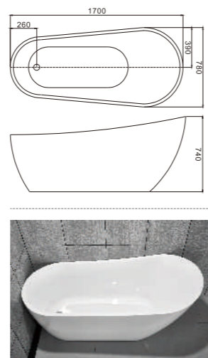
C-3225 Size:780x1700x740/mm
