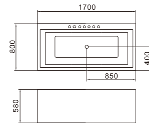
C-476 Size:800x1700x580/mm
