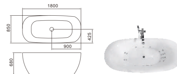
C-3227 Size:850x1800x680/mm
