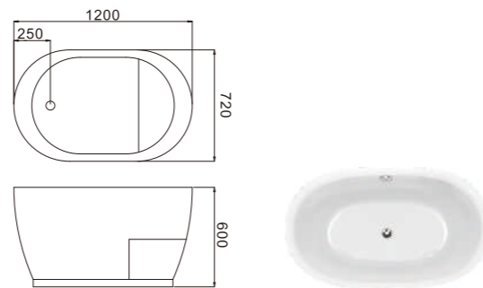
C-3249 Size:720x1200x600/mm
