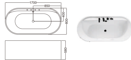
C-3229-HLT Size:800x1700x580/mm
