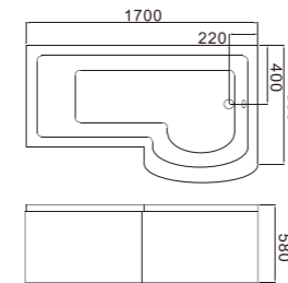
C-482-17(L) Size:800x1700x580/mm
