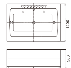
C-480 Size:1200x1700x580/mm
