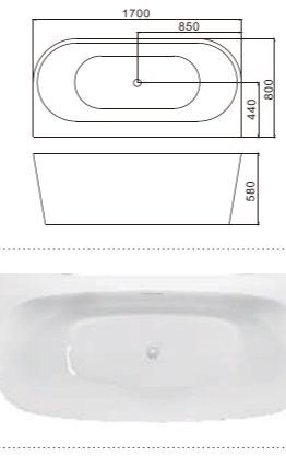
C-3243 Size:800x1700x580/mm
