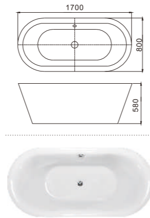
C-3252-B-17 Size:800x1700x580/mm
