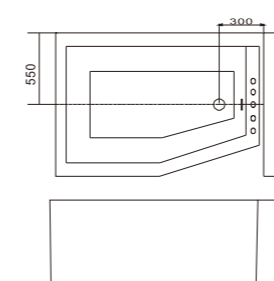
C-484(L) Size:1200x1700x580/mm
