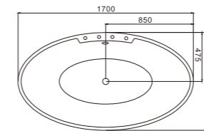
C-3217 Size:950x1700x580/mm
