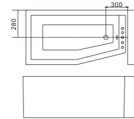
C-483-17(L) Size:800x1700x580/mm
