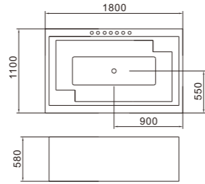
C-473 Size:1100x1800x580/mm
