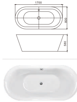
C-3252-17 Size:800x1700x580/mm
