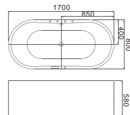
C-3165 Size:800x1700x580/mm
