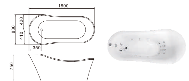
C-3228 Size:830x1800x750/mm
